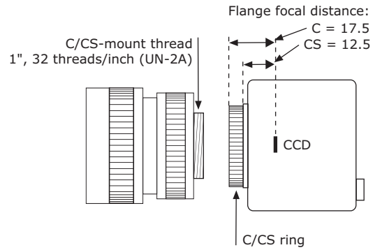
Fig. 3: The C-mount thread.
